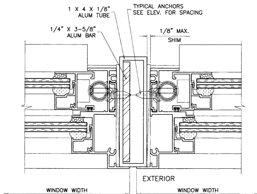
MULLION TYPE '2'
