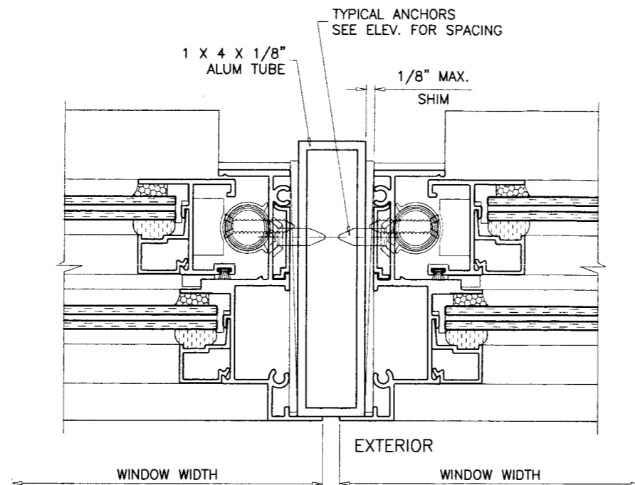
MULLION TYPE '1'
